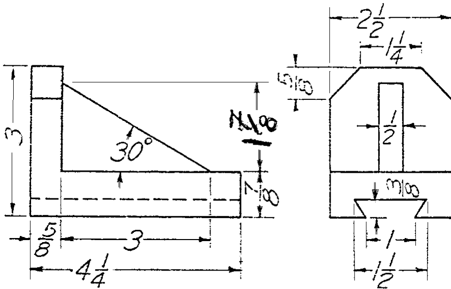
Prob. 5.1.5 Dovetail stop
