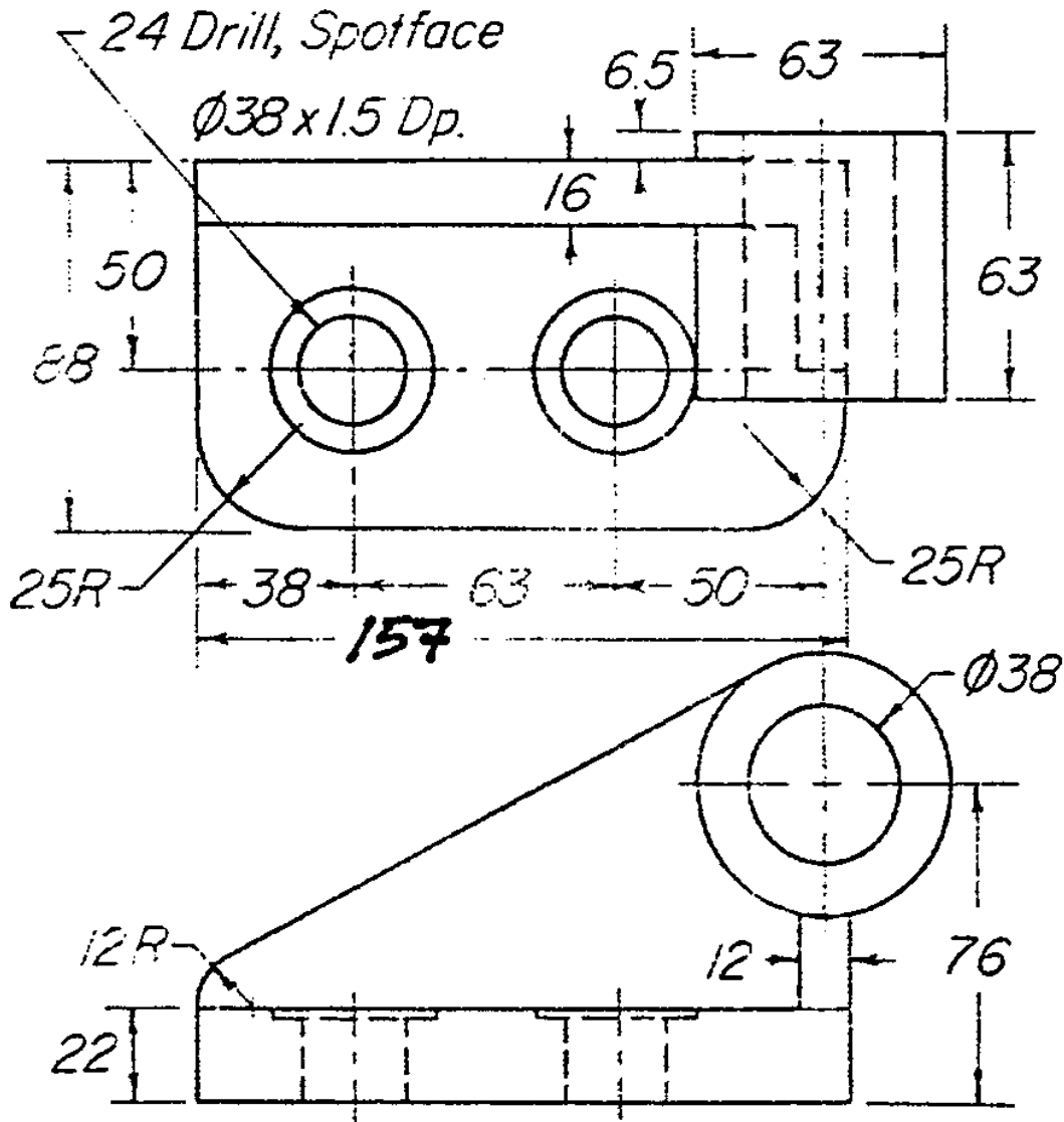
Prob. 5.1.9 METRIC Offset
