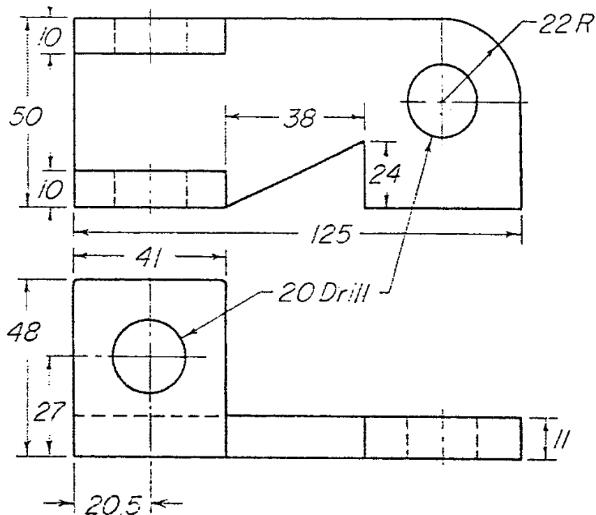
Prob. 5.1.6 METRIC Hinged catch
