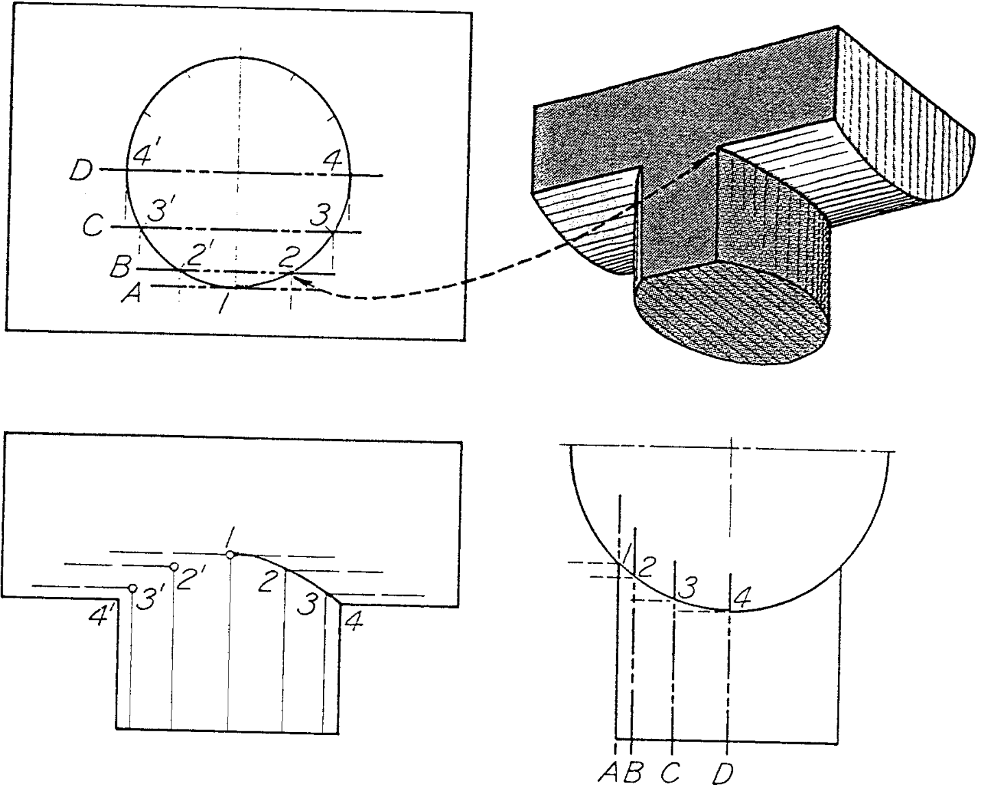
Fig. 11.16 Intersection of two cylinders
