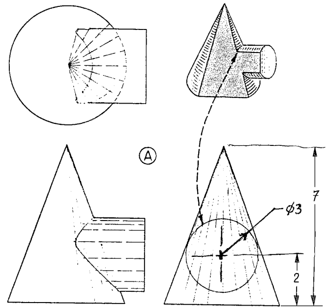
Fig. 11.19 Intersection of a cylinder and cone.
