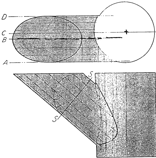
Fig. 11.17 Intersection of two cylinders, axes not intersecting
