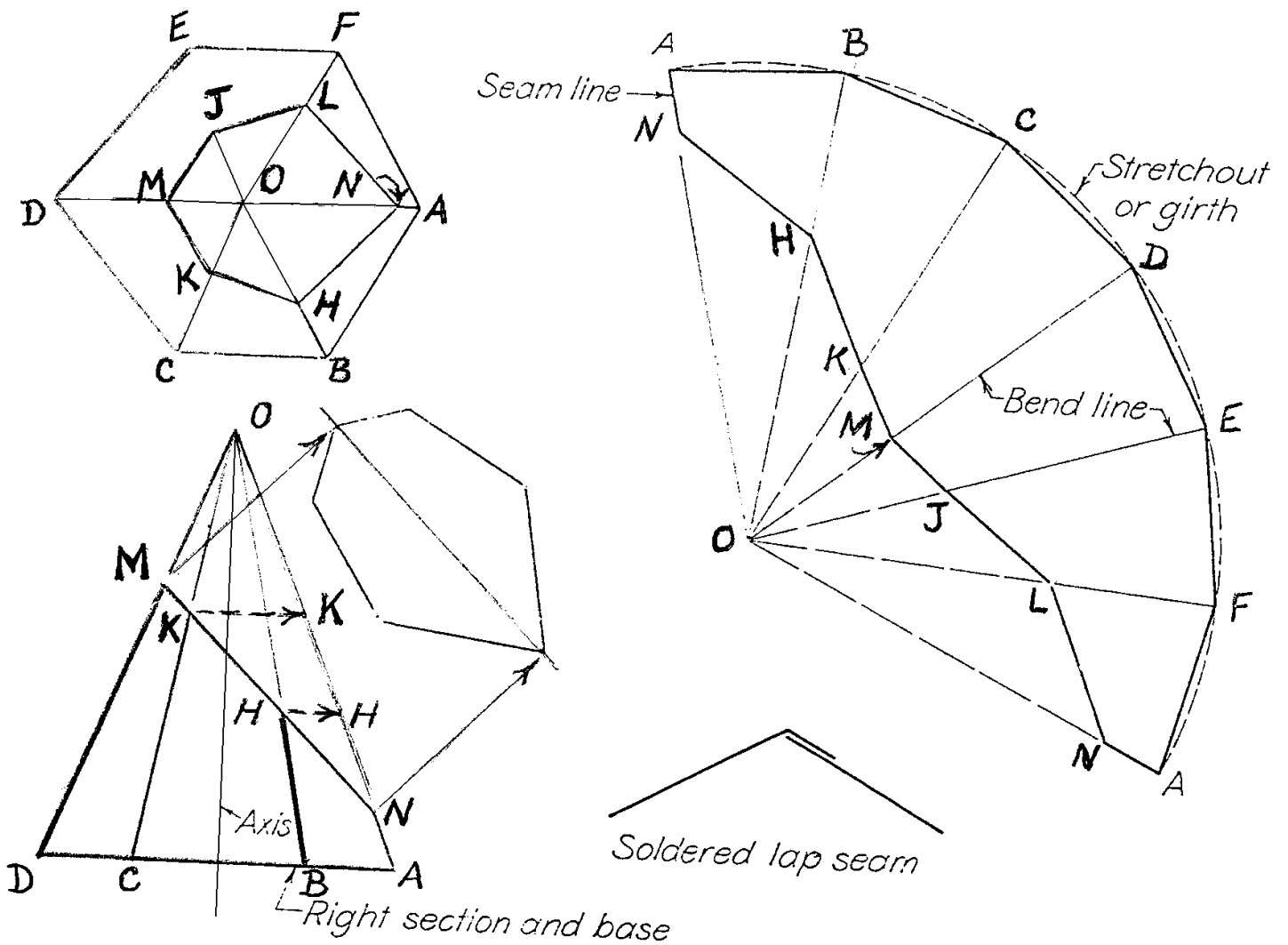
2.9 Development of a pyramid
