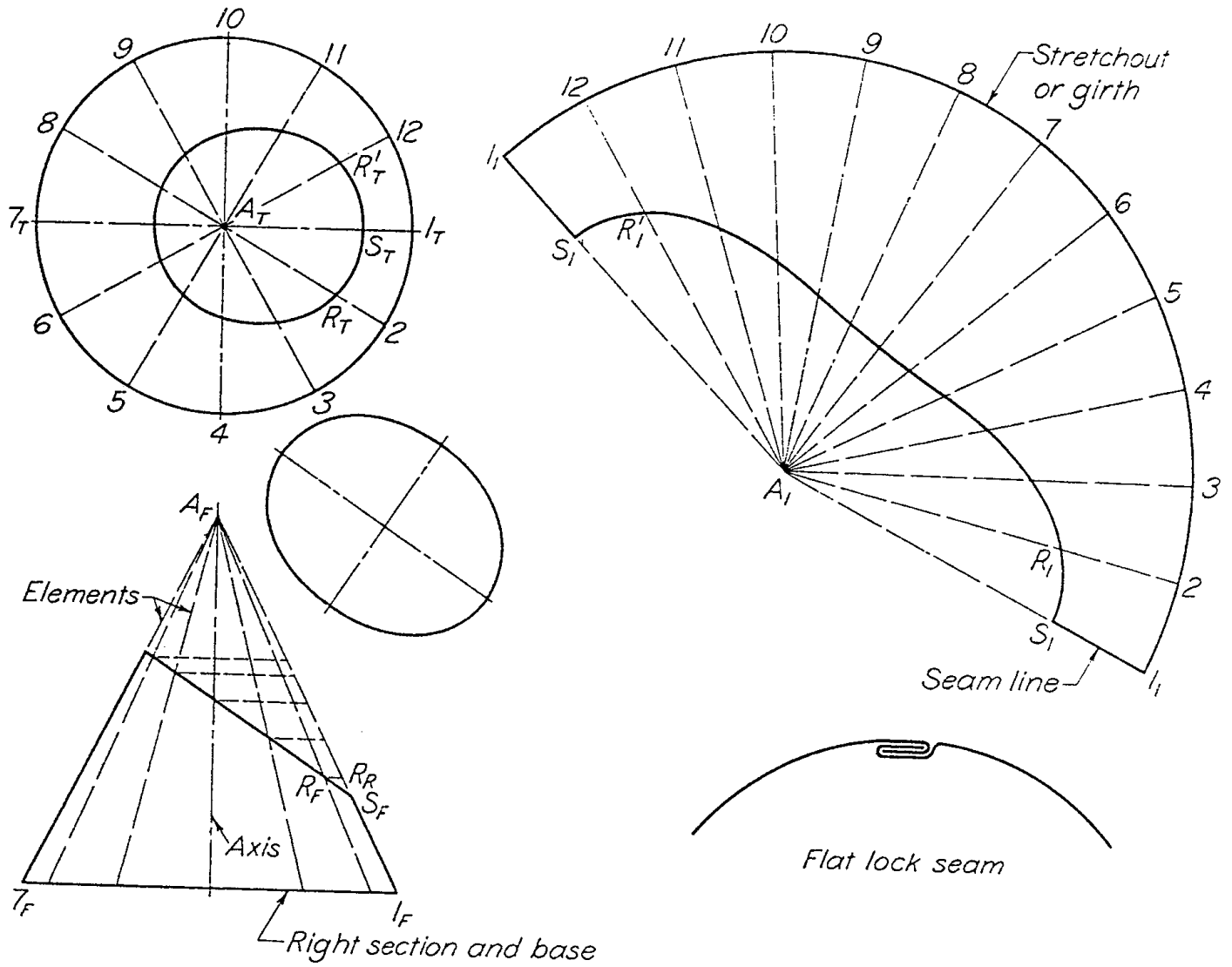
Fig. 12.13 Development of a cone
