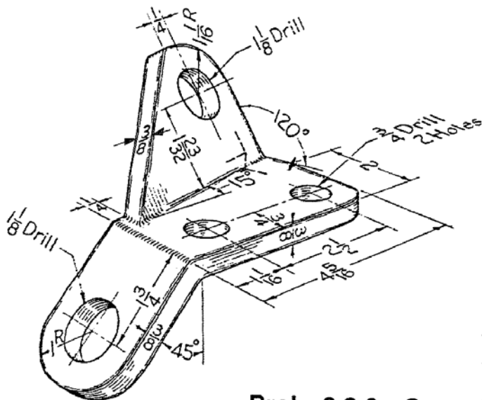
Prob. 8.2.6 Spar clip
