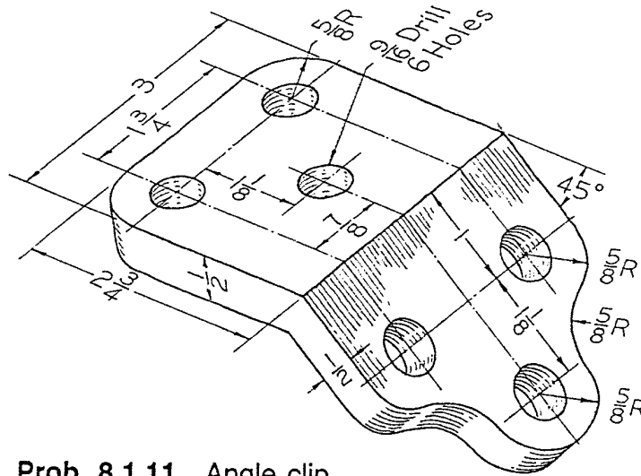
Prob. 8.1.11 Angle clip
