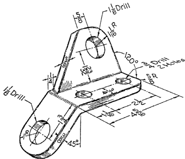
Prob. 8.1.17 Spar clip, 120°
