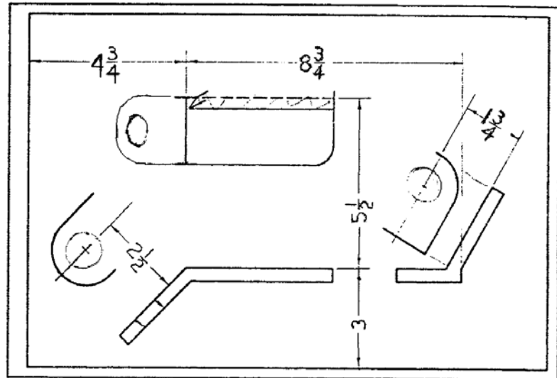
Prob. 8.1.17 Spar clip, 120°
