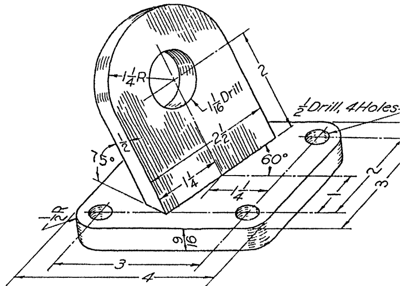
Prob. 8.2.2 Anchor base
