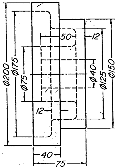
Prob. 6.1.3 METRIC. Step pulley.
