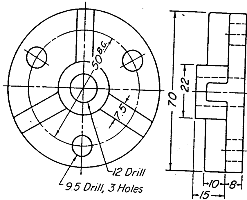
Prob. 6.1.7 METRIC. Ribbed support.
